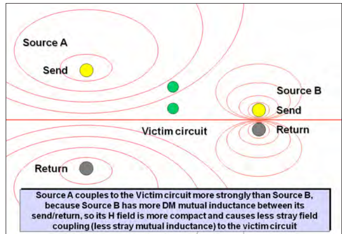
Figure 6. Example of H-field coupling.
